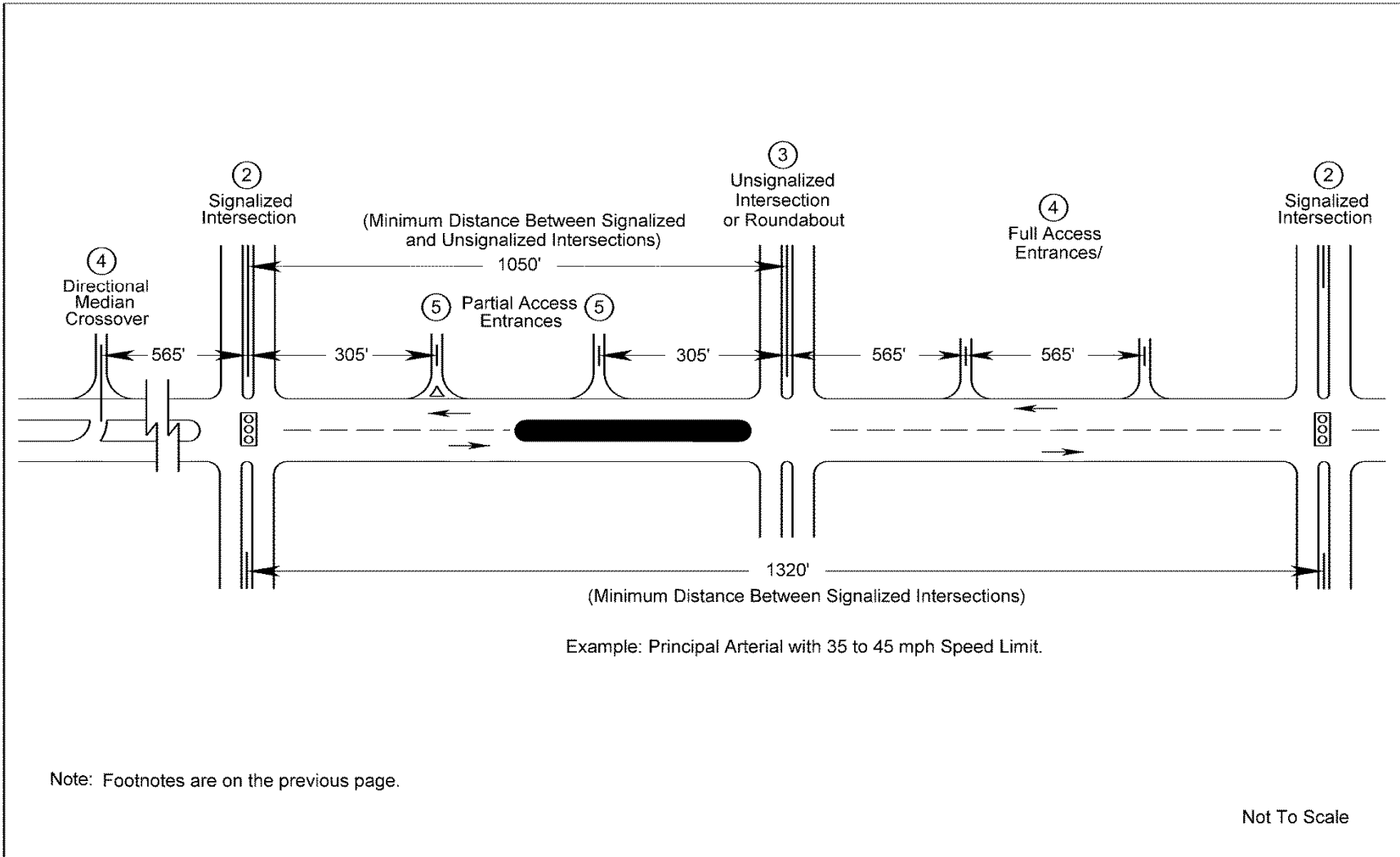
FIGURE 2-8.1 ILLUSTRATION OF THE RELATIONSHIP BETWEEN SPACING STANDARDS*
