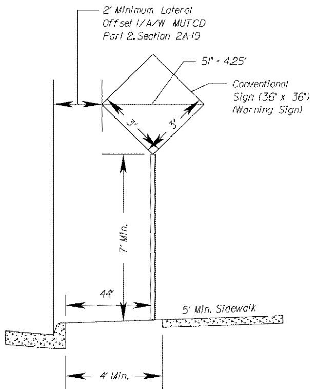
Typical Urban Projects 25 mph Posted Speed and Greater
