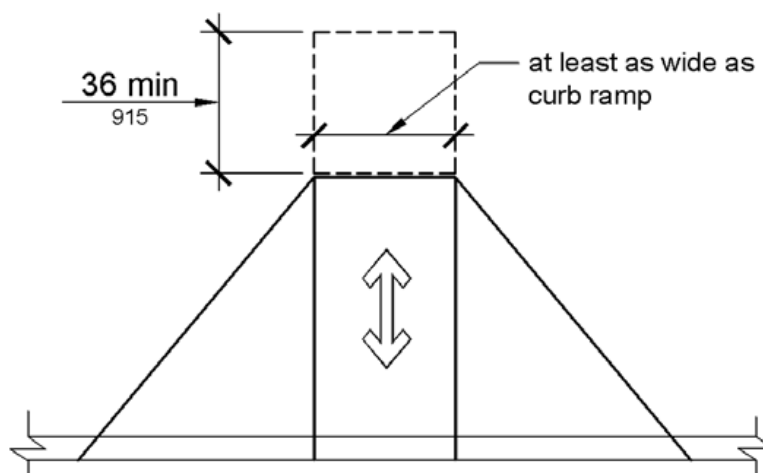
LANDINGS AT THE TOP OF CURB RAMP*
