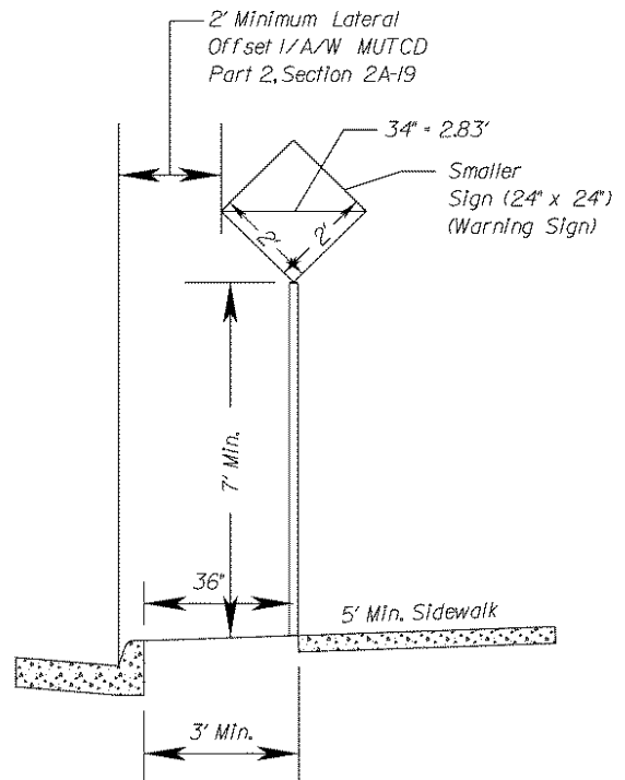
Subdivision Streets 25 mph Posted Speed and Less
