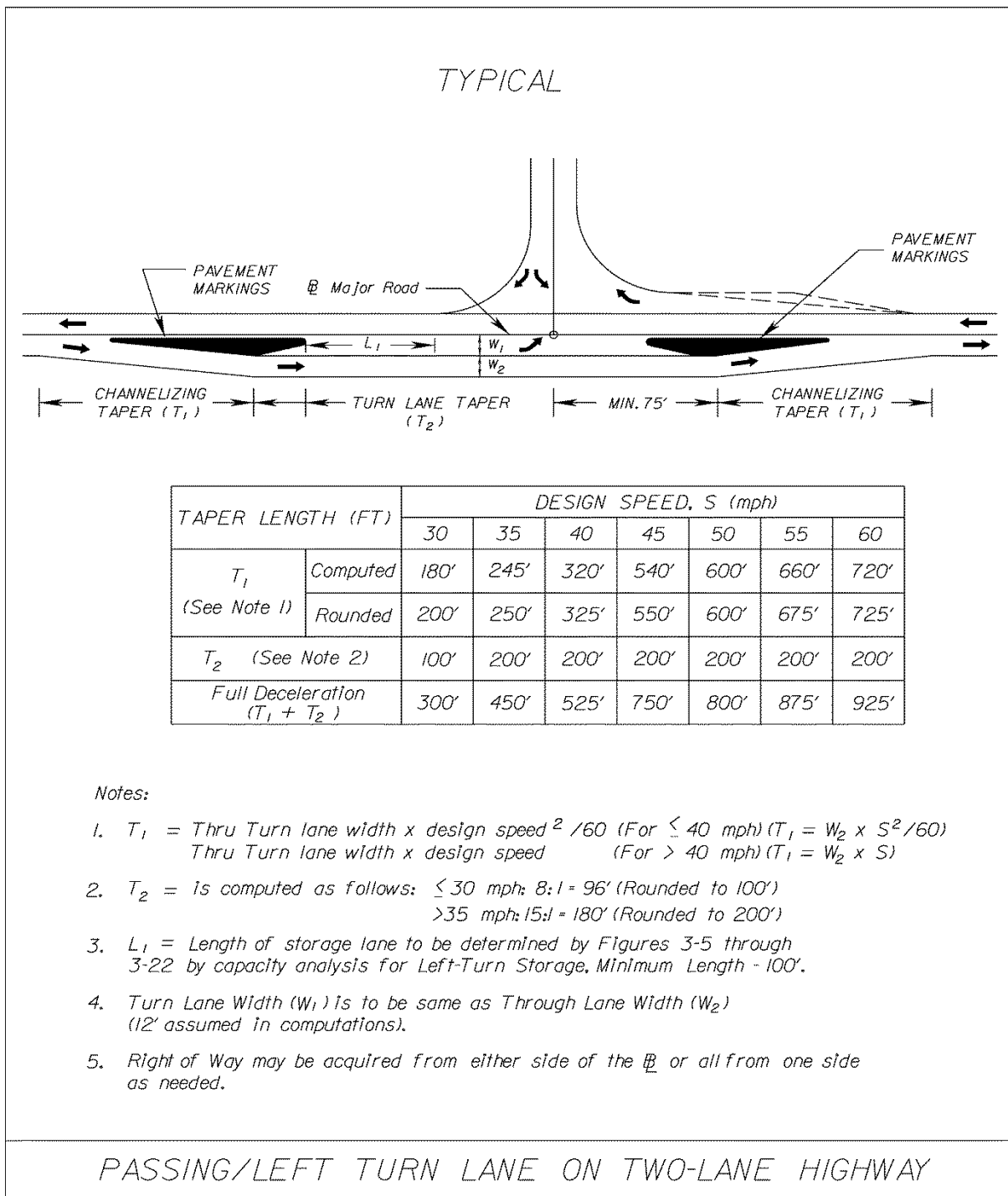
FIGURE 3-4 PASSING/LEFT TURN LANE ON TWO-LANE HIGHWAY
