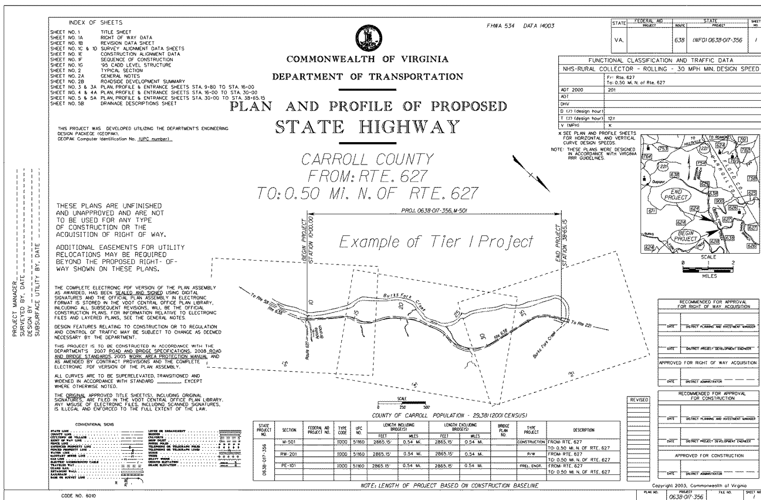
FIGURE 2E-12 SAMPLE TITLE SHEET (SECONDARY DESIGN) TIER 1*
