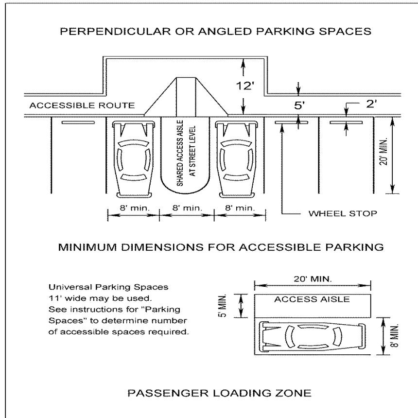
FIGURE C-1-3 ACCESSIBLE PARKING AND LOADING ZONES*
