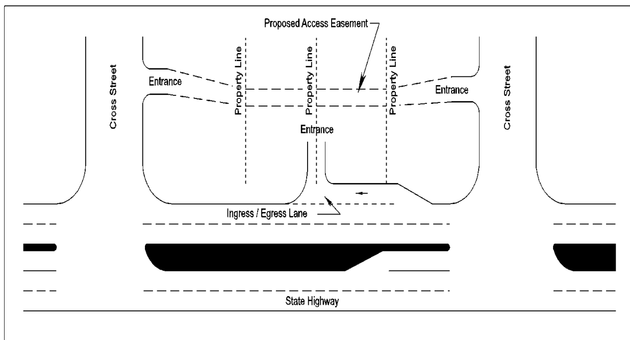
FIGURE 2-2 VEHICULAR CIRCULATION BETWEEN ADJOINING PROPERTIES
