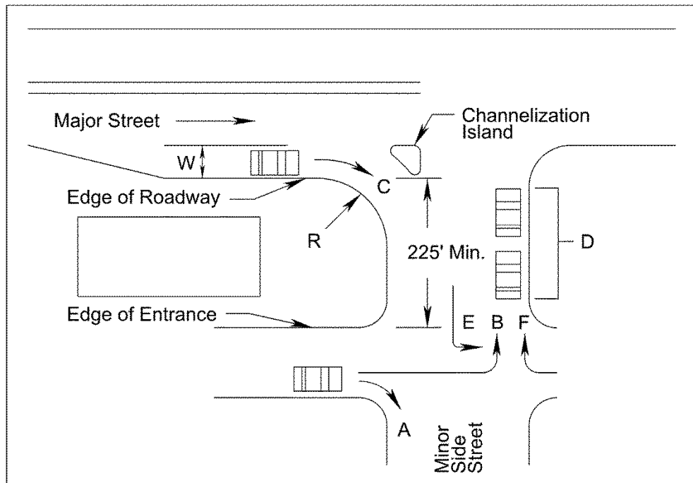
FIGURE 4-5 CORNER CLEARANCE
