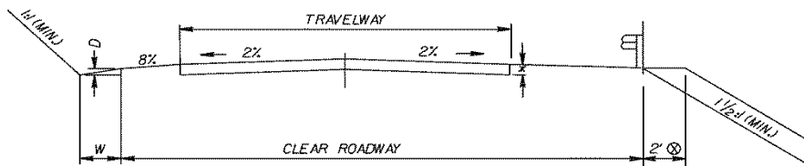
TYPICAL SECTION
