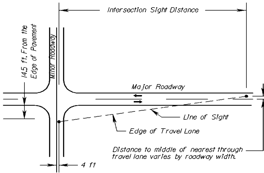
Right Sight Distance Triangle
