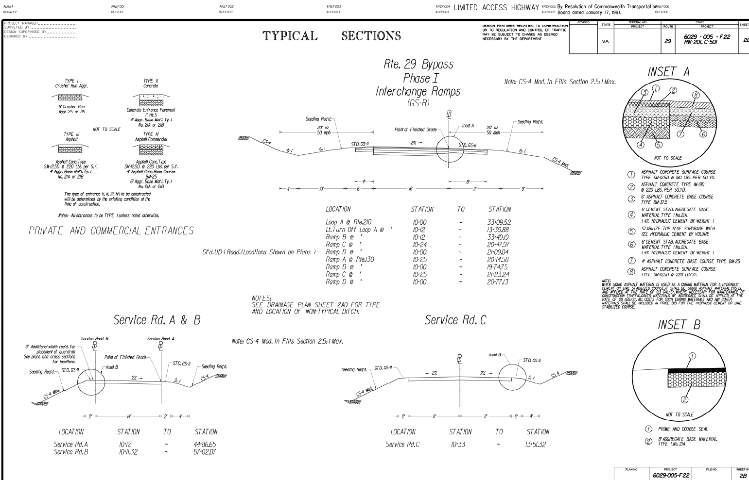
FIGURE 2E-18.1 SAMPLE TYPICAL SECTION SHEET*
