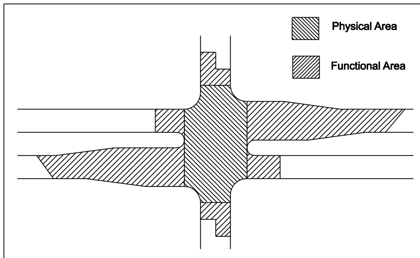
FIGURE 4-2A PHYSICAL AND FUNCTIONAL AREAS OF INTERSECTION
