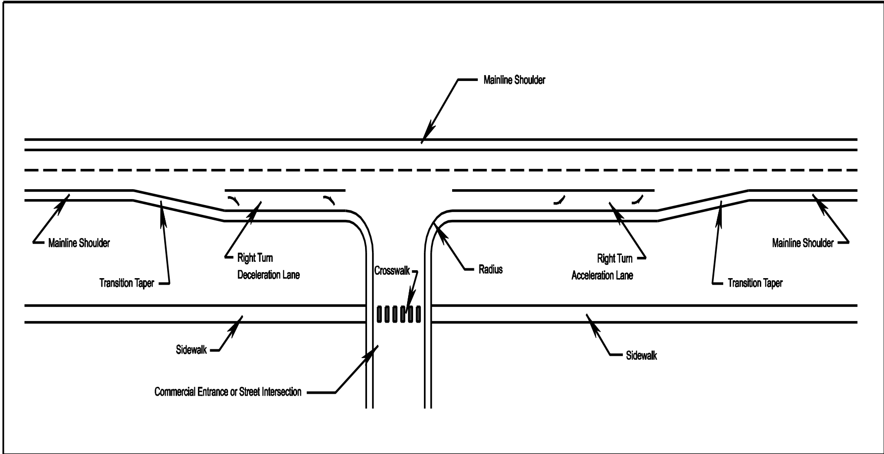
FIGURE 3- 32 TYPICAL APPLICATION OF A RIGHT TURN ACCELERATION AND DECELERATION LANE (SHOULDER SECTION)
