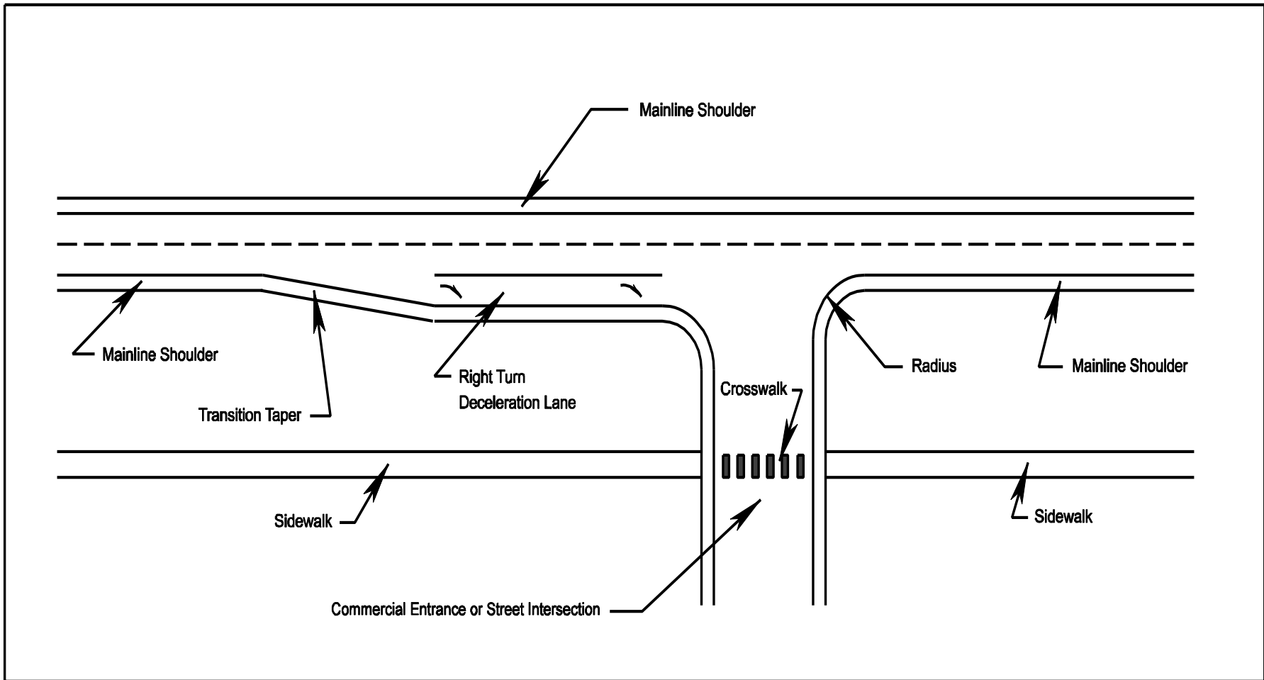
FIGURE 3-30 TYPICAL APPLICATION OF A RIGHT TURN DECELERATION LANE (SHOULDER SECTION)
