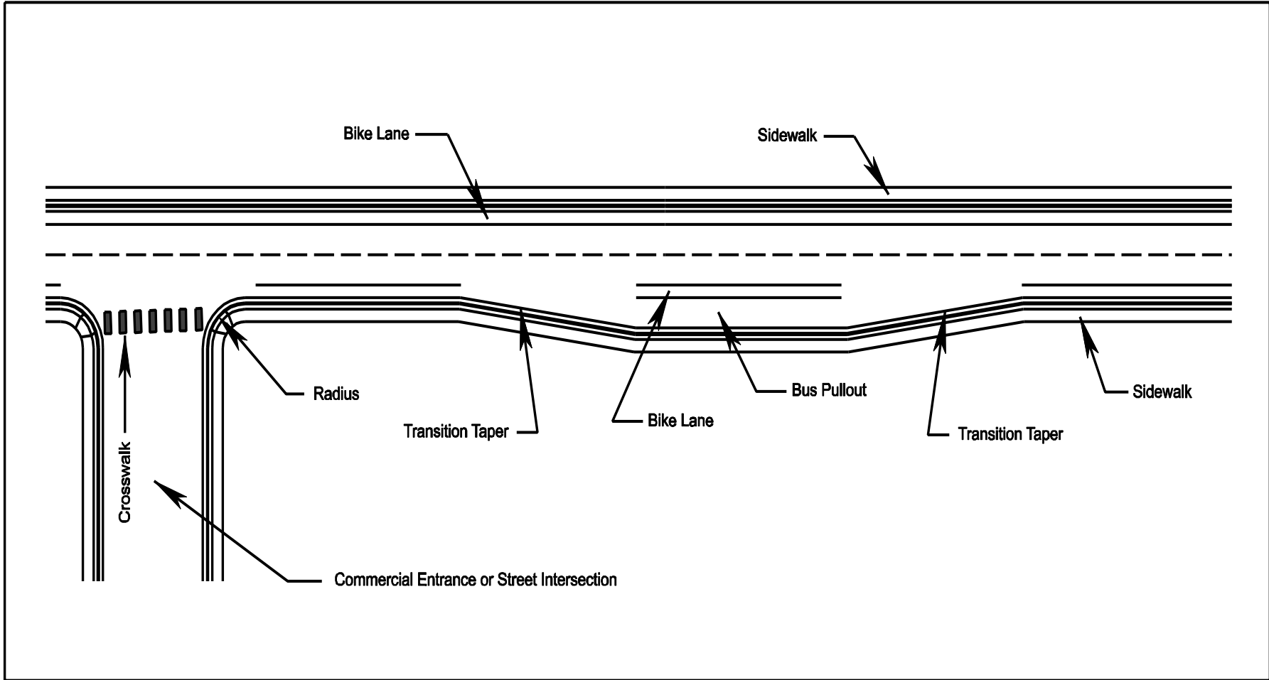
FIGURE 3- 29 TYPICAL APPLICATION OF A BUS PULLOUT
