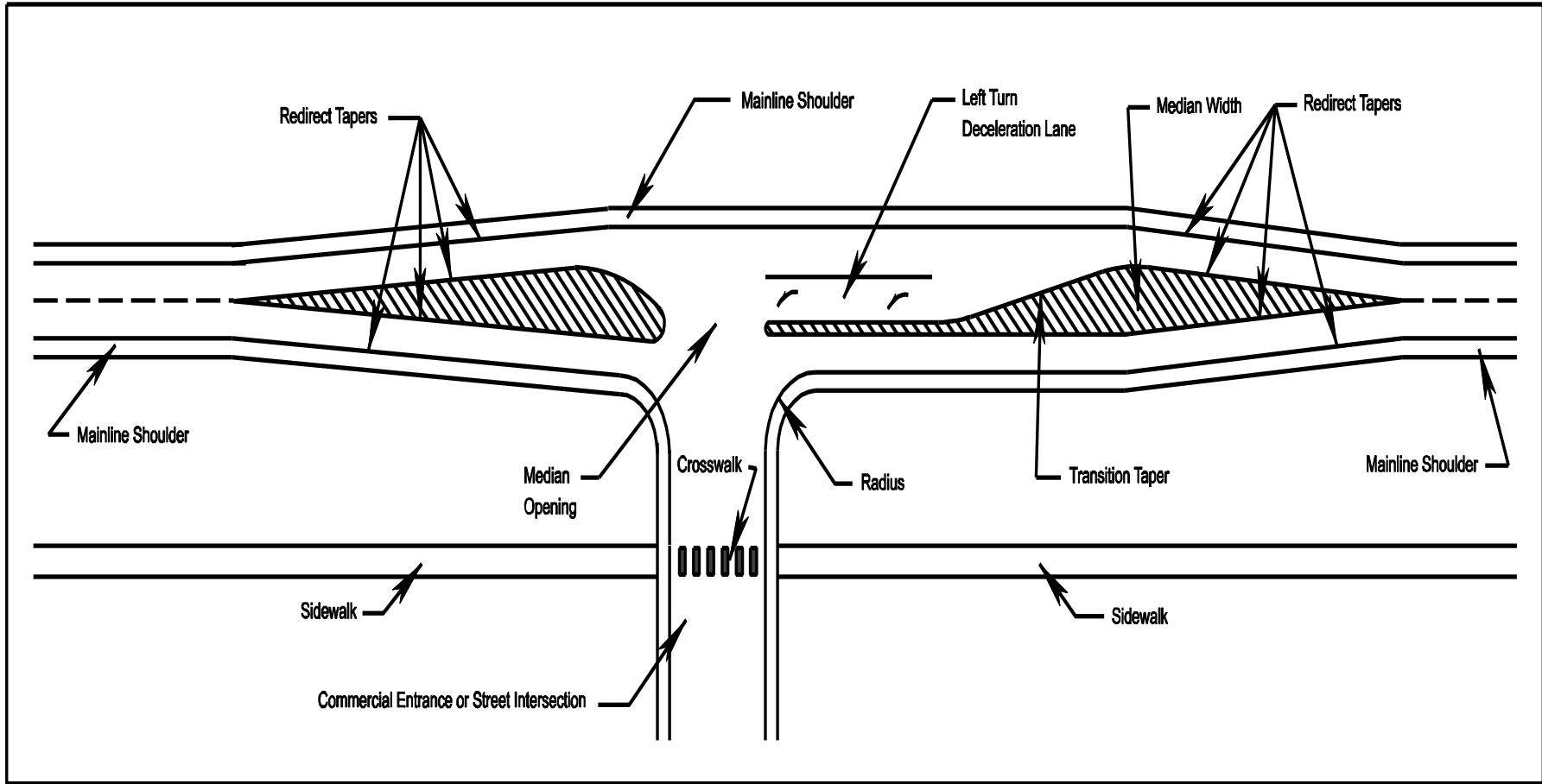
FIGURE 3-31 TYPICAL APPLICATION OF A LEFT TURN DECELERATION LANE (SHOULDER SECTION)
