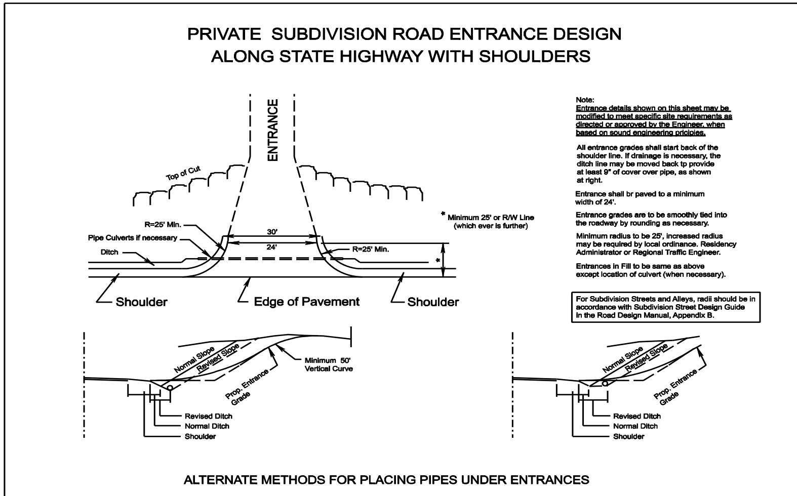
FIGURE 4- 8 STANDARD PRIVATE SUBDIVISION ROAD / STREET ENTRANCE
