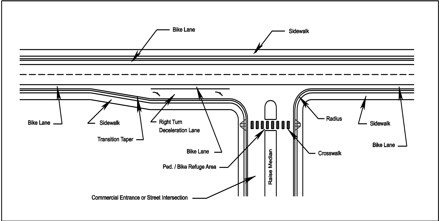
FIGURE 3-28 TYPICAL APPLICATION WITH SIDEWALKS AND BIKE LANES WITH RIGHT-TURN DECELERATION LANES (CURB AND GUTTER SECTION)
