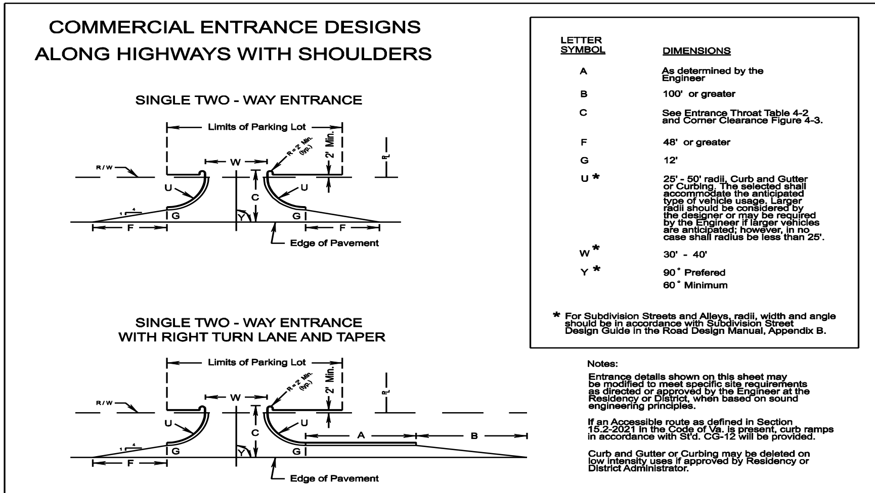
FIGURE 4- 9 COMMERCIAL ENTRANCE DESIGNS ALONG HIGHWAYS WITH SHOULDERS
