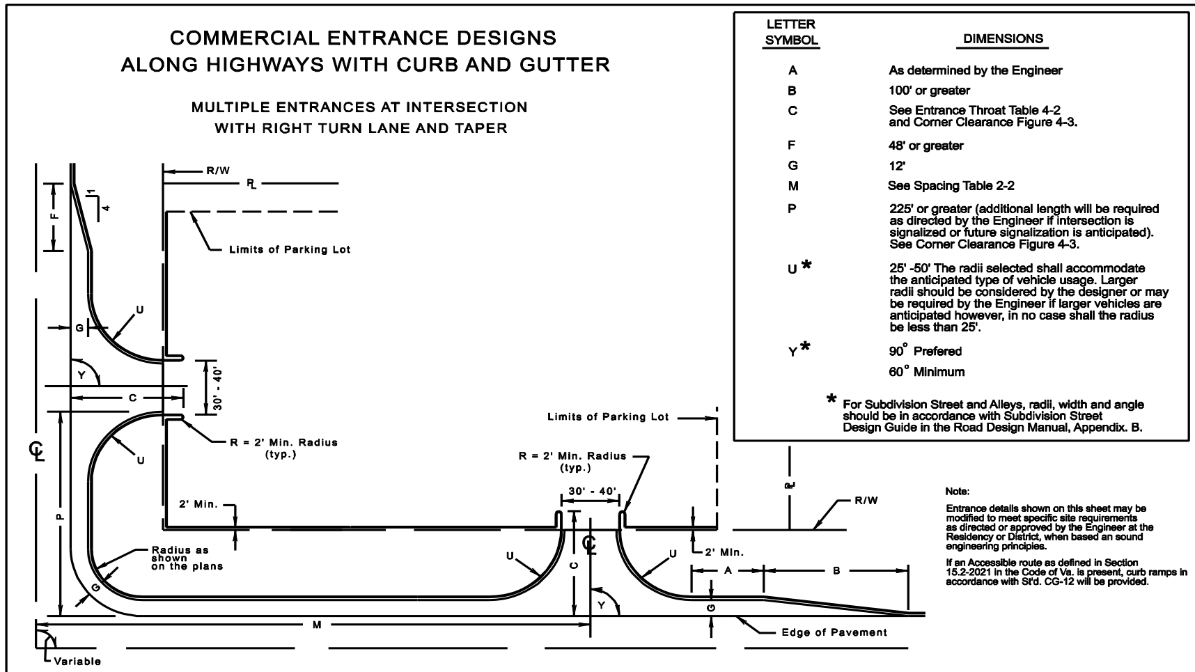
FIGURE 4-13 COMMERCIAL ENTRANCE DESIGNS ALONG HIGHWAYS WITH CURB AND GUTTER AT INTERSECTION
