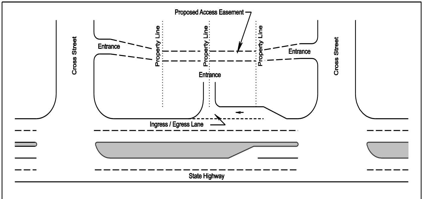
FIGURE 2-2 VEHICULAR CIRCULATION BETWEEN ADJOINING PROPERTIES
