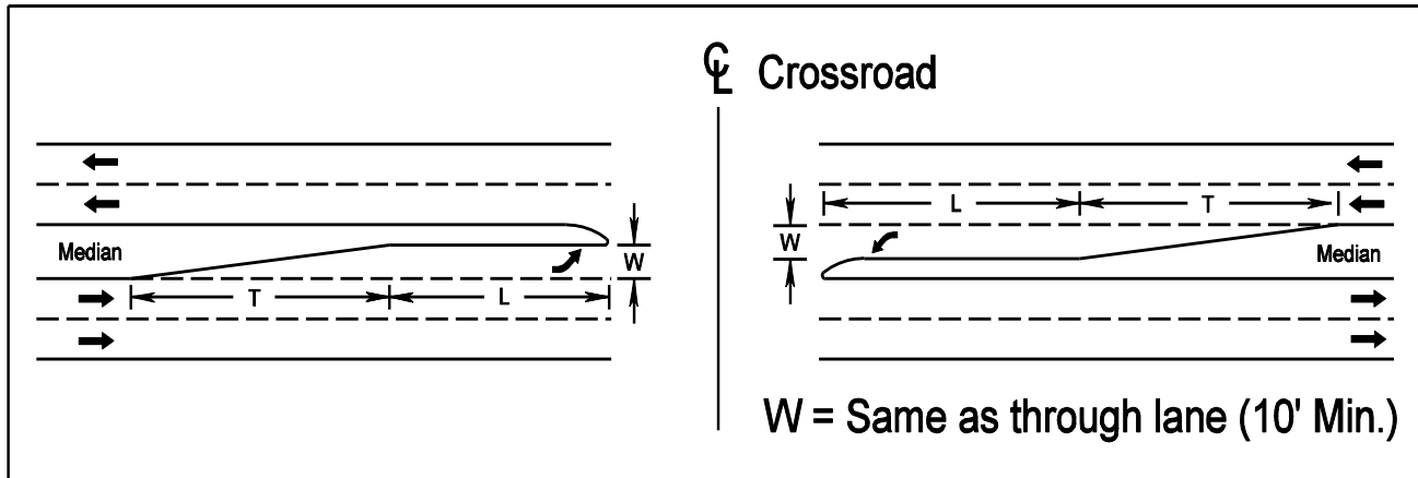
FIGURE 3-2 LEFT AND RIGHT TURN STORAGE AND TAPER LENGTHS
