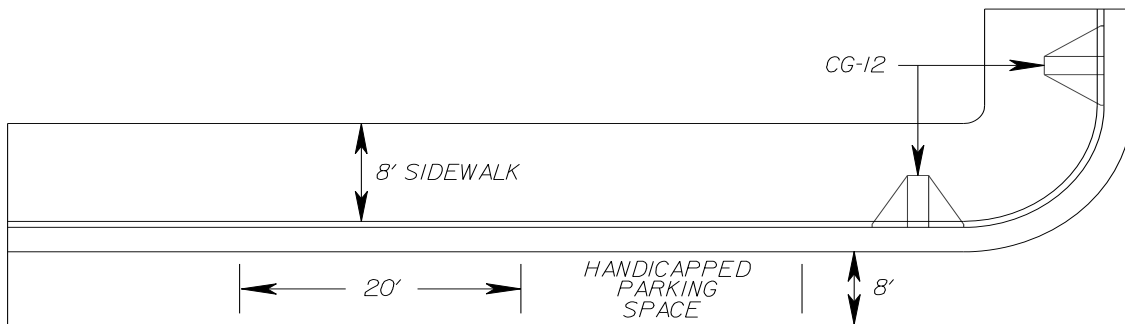
FIGURE C-1-2 DESIGNS FOR PARALLEL PARKING SPACES EXCEPTION
