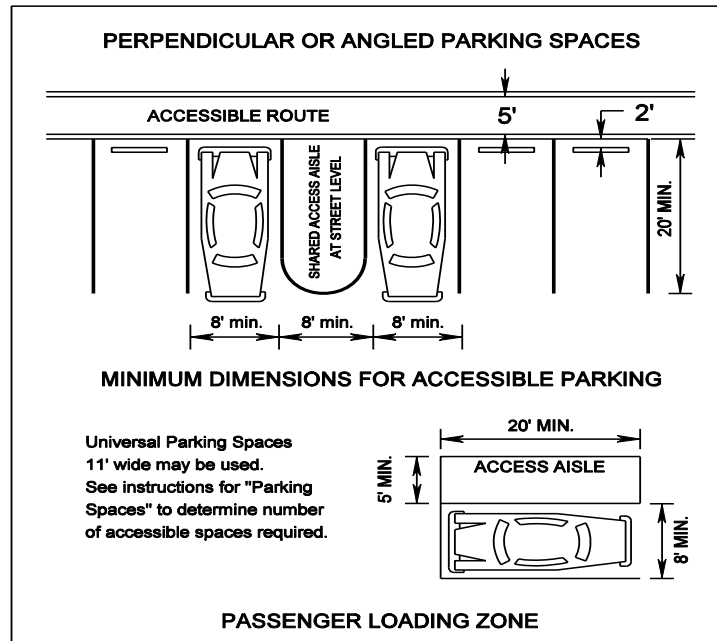
FIGURE C-1-3 ACCESSIBLE PARKING AND LOADING ZONES
