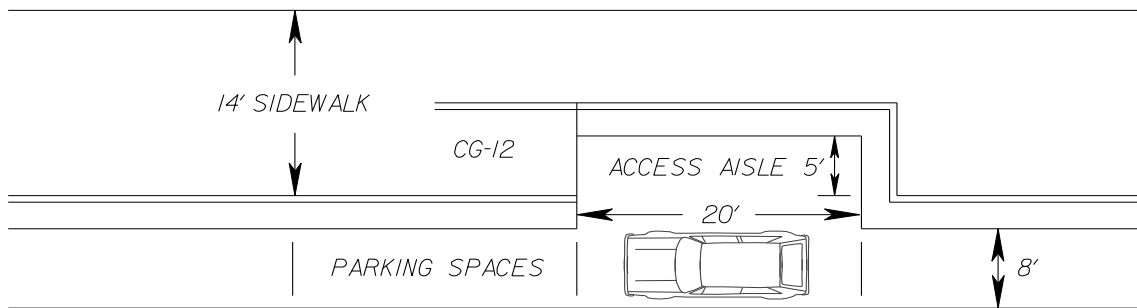
FIGURE C-1-1 DESIGNS FOR PARALLEL PARKING SPACES
