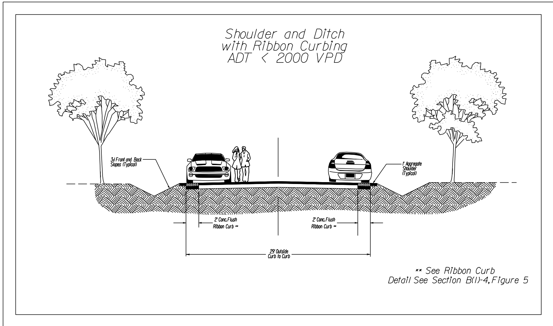
FIGURE 1.8 – 29' STABILIZED SHOULDER AND DITCH WITH RIBBON CURB*
