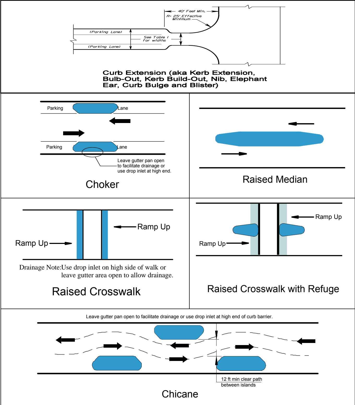
FIGURE 12 – TRAFFIC CALMING DETAILS*
