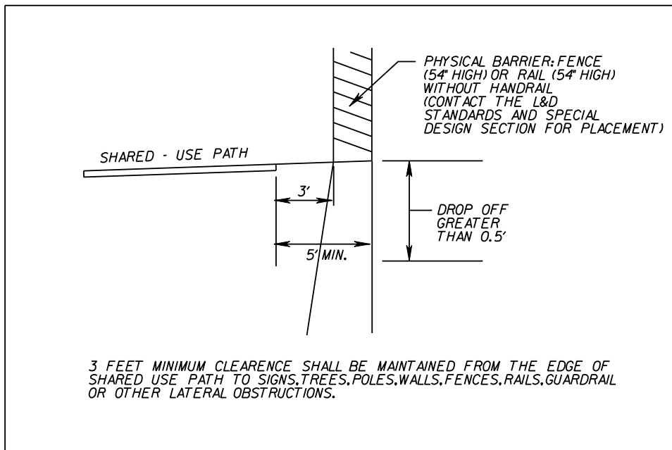
FIGURE A-5-7 PHYSICAL BARRIER FOR SHARED-USE PATH
