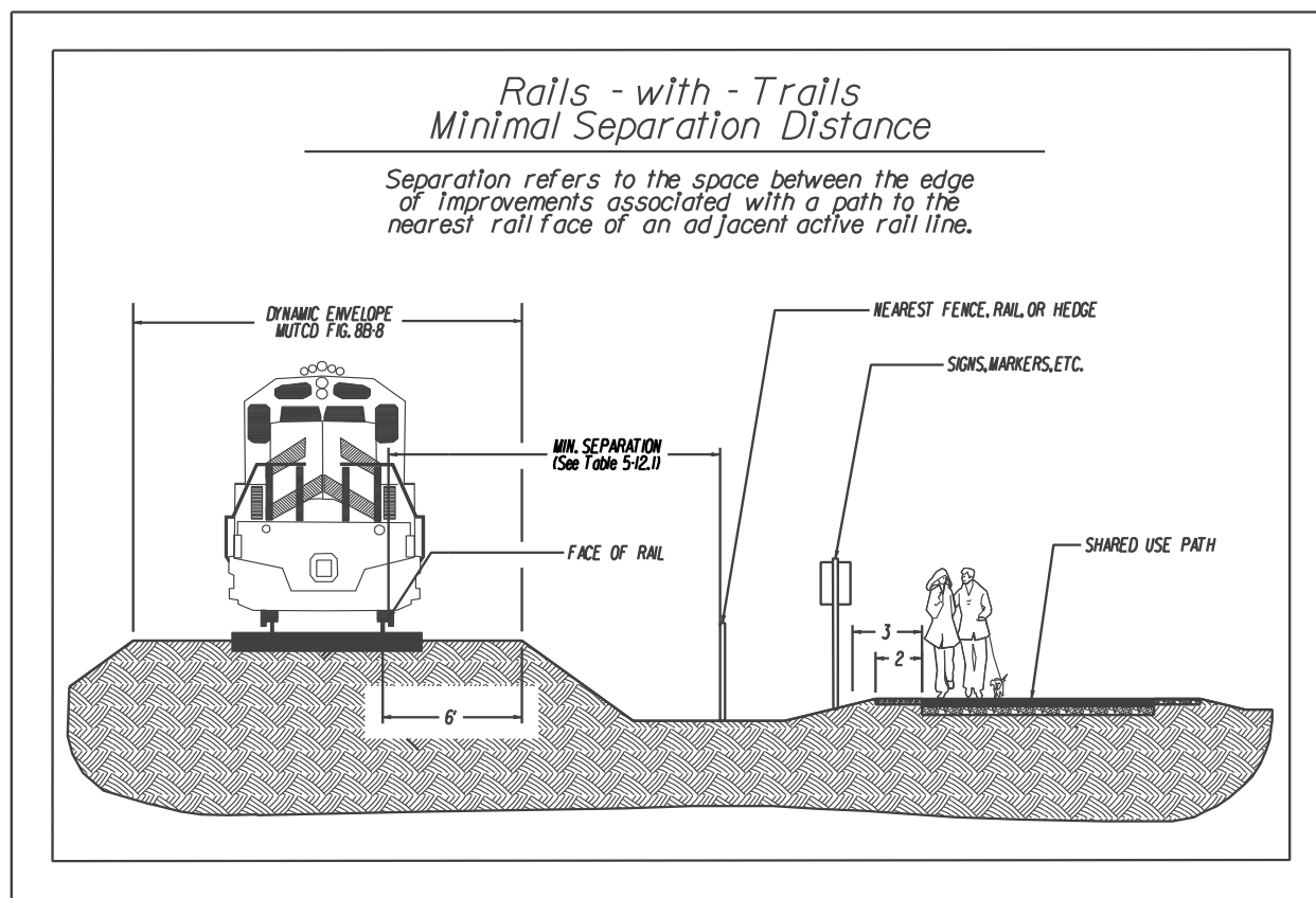
FIGURE A- 5-10 SEPARATION BETWEEN ACTIVE RAIL LINES AND PATHS (RWT)
