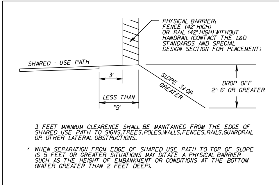
FIGURE A-5-6 PHYSICAL BARRIER FOR SHARED-USE PATH*
