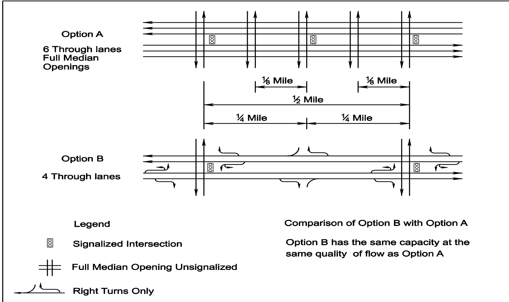
FIGURE 2-8 ILLUSTRATION OF ENTRANCE AND INTERSECTION SPACING
