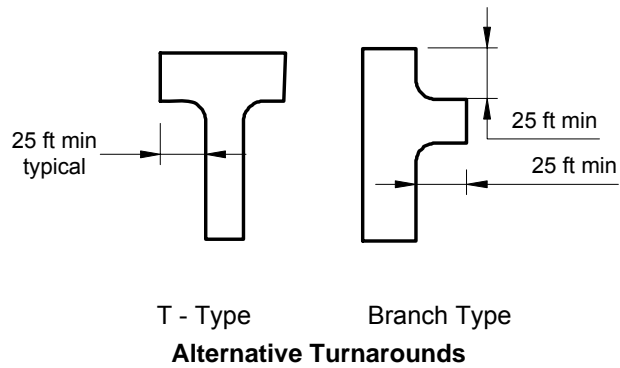
FIGURE 4 – CUL-DE-SAC DETAILS*
