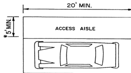
MINIMUM DIMENSIONS FOR ACCESSIBLE PARKING
