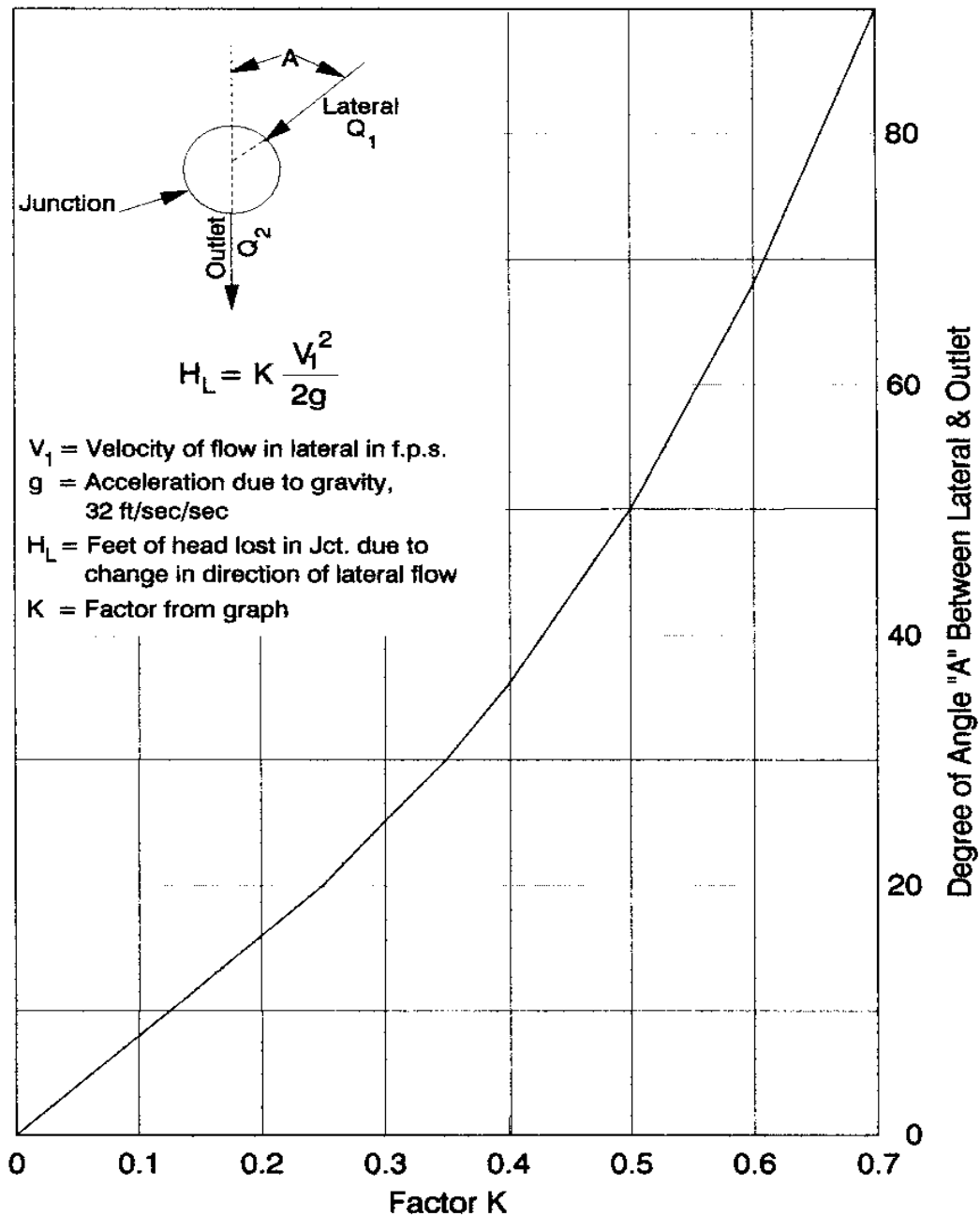
Figure 9-9. Losses in Junction Due to Change in Direction of Flow Lateral
