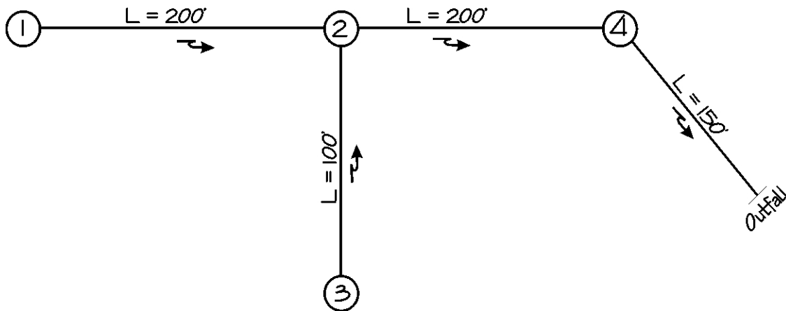
Figure 9-10*. Storm Drain Layout Sample Problem
