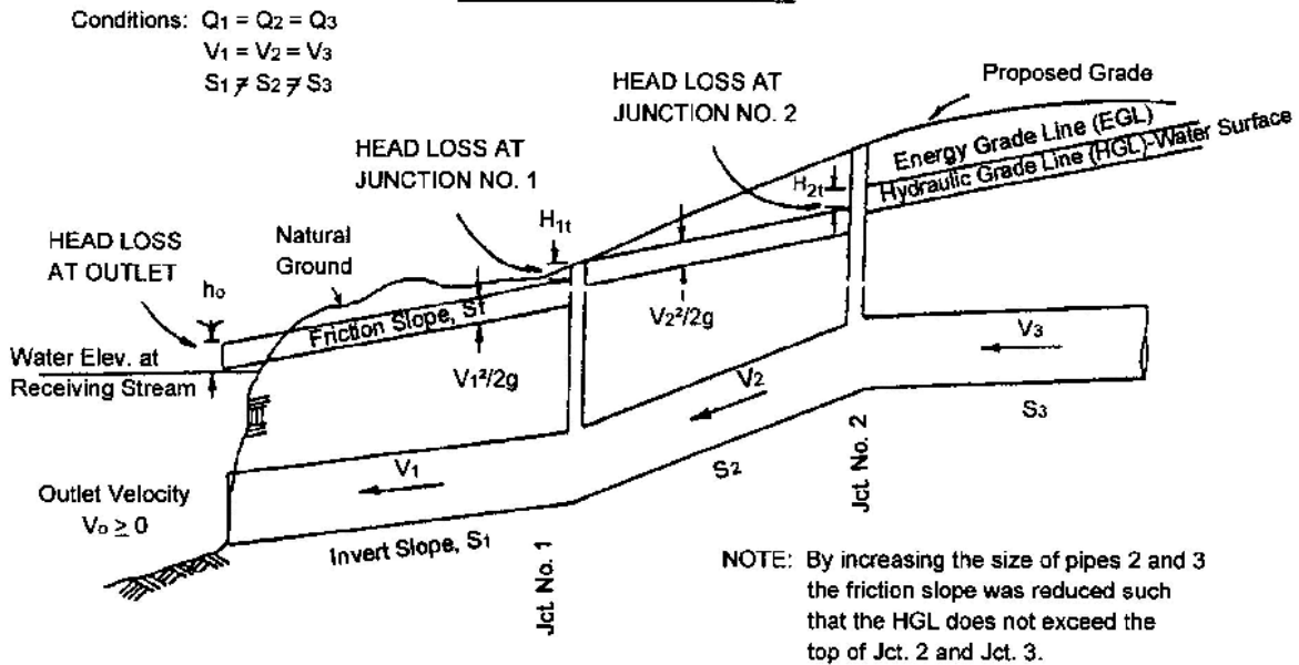
Figure 9-7. Use of Energy Losses in Analyzing a Storm Drain System
