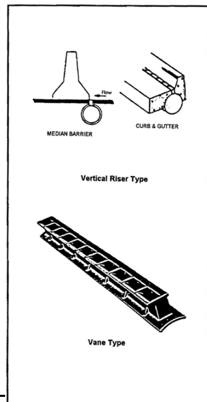
Figure 9-4. Slotted Drain Inlets
