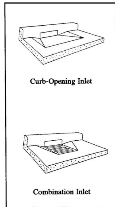
Figure 9-3. Curb Inlets
