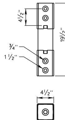
X4-HINGE ASSEMBLY
