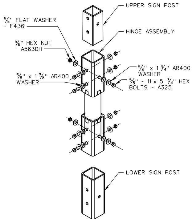
HINGE INSTALLATION DETAIL
