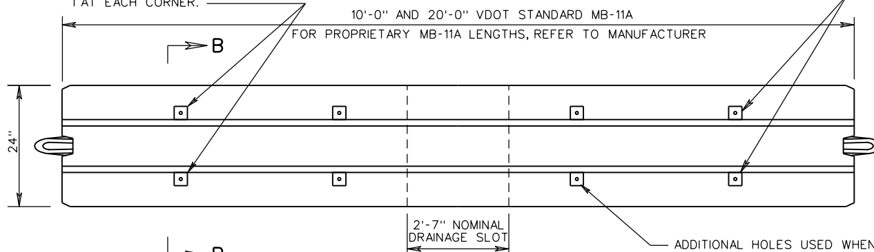
PLAN VIEW
