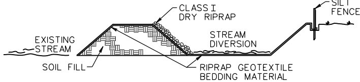
DAM DETAIL
