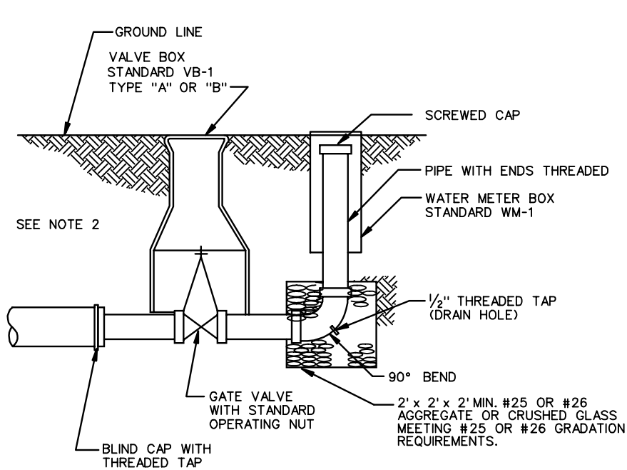
TYPE "A"
