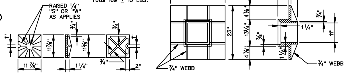
TYPE "C"
