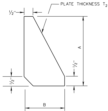
STIFFENER PLATE
