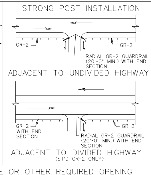
INSTALLATION AT ENTRANCE OR OTHER REQUIRED OPENING
