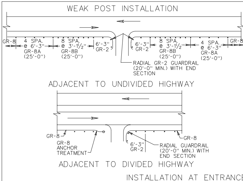
INSTALLATION AT ENTRANCE OR OTHER REQUIRED OPENING
