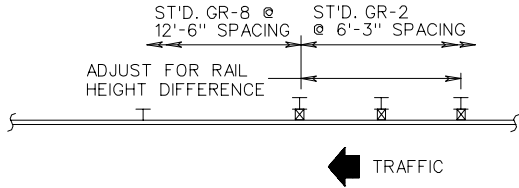
TRANSITION FROM STRONG POST TO WEAK POST GUARDRAIL
