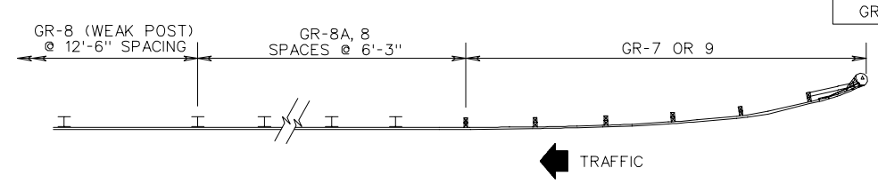
TRANSITION FROM GR-7 & GR-9 TERMINAL TO WEAK POST GUARDRAIL
