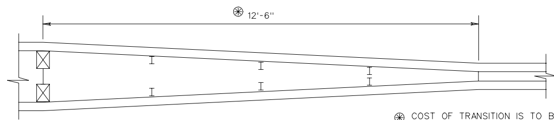
DETAIL A
