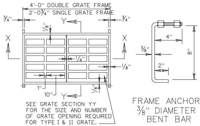
GRATE AND FRAME PLAN
