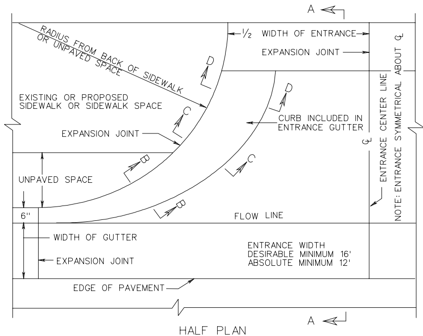
HALF PLAN
