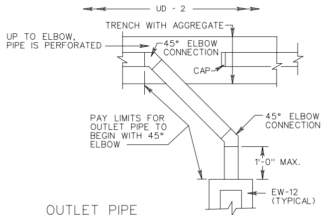
OUTLET PIPE
