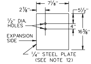
ANCHOR SLAB TYPE II END PLATE DETAIL
