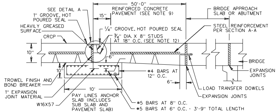
SECTION F-F ANCHOR SLAB TYPE II
