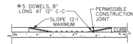
SECTION B-B
