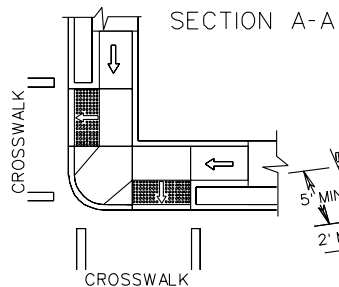
TYPICAL PLACEMENT AT INTERSECTION WITH BUFFER STRIP
