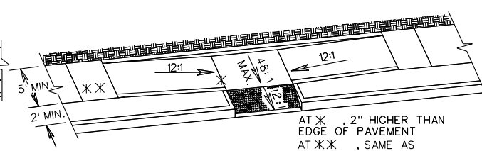
TYPE C (PARALLEL & PERPENDICULAR) APPLICATION
