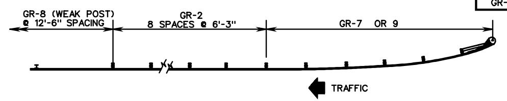
TRANSITION FROM GR-7 & GR-9 TERMINAL TO WEAK POST GUARDRAIL
