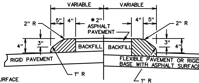
ASPHALT MEDIAN
