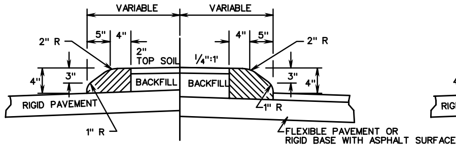
ASPHALT MEDIAN
