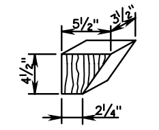
ITEM 10 DETAIL
