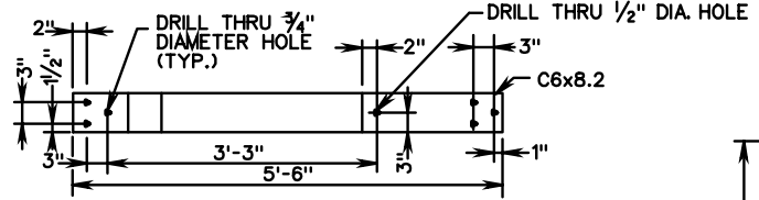
ITEM 8 DETAIL
