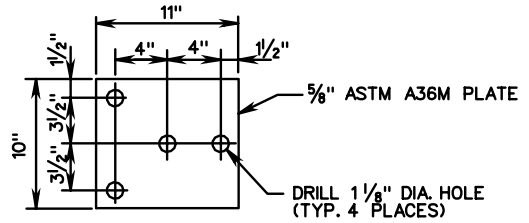
BEARING PLATE
