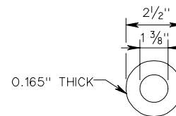
PLAIN GALVANIZED STEEL WASHER FOR 1 1/4" PIN
