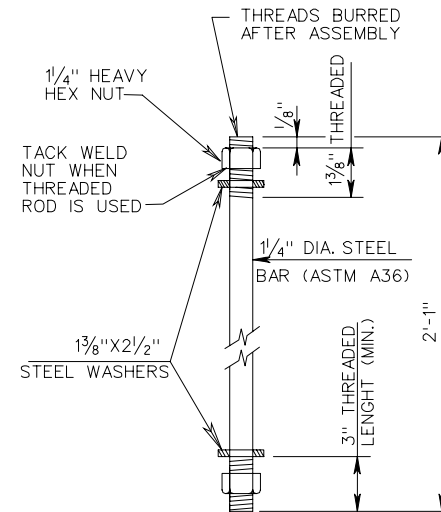
CONNECTOR PIN ASSEMBLY GALVANIZE AFTER FABRICATION.
