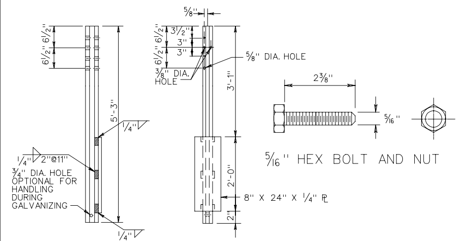
S 3 X 5.7 STEEL POST
