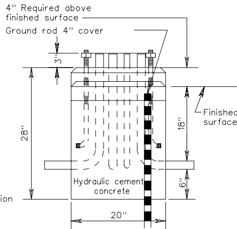
TYPICAL FOUNDATION DETAIL
