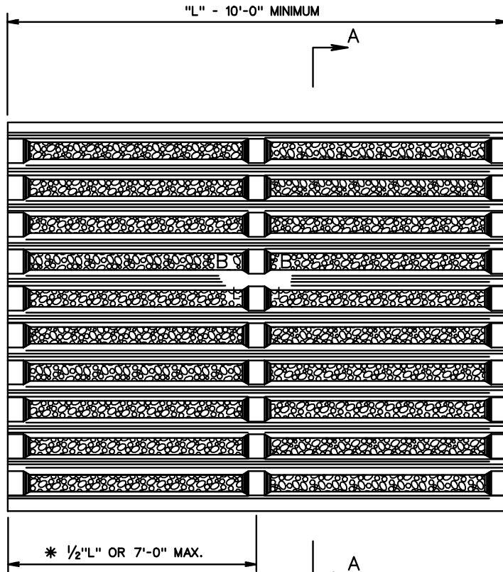
PLAN VIEW
