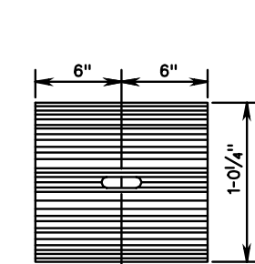
W BEAM BACK-UP PLATE
