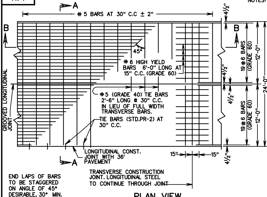
PLAN VIEW
