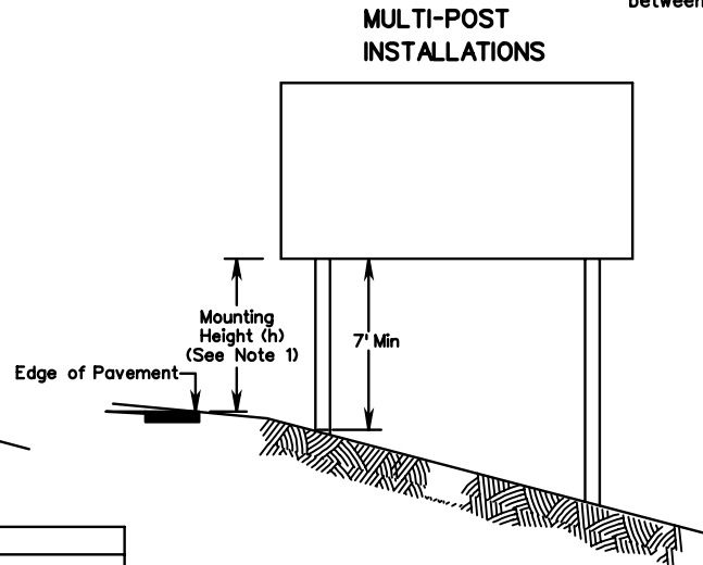
INSTALLATION DETAILS
