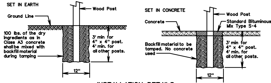
INSTALLATION DETAILS
