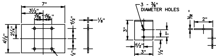
ANTI-TWIST PLATE
