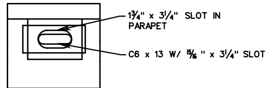
ALTERNATE SLOT DETAIL
