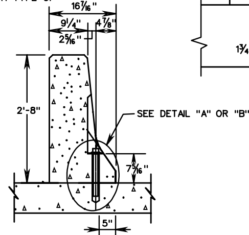
SECTION B-B (ANCHOR BOLT)
