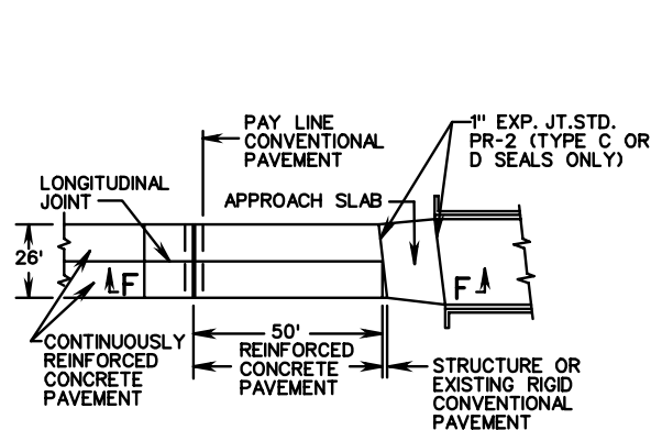
PLAN VIEW ANCHOR SLAB TYPE II (SEE NOTE 11)
