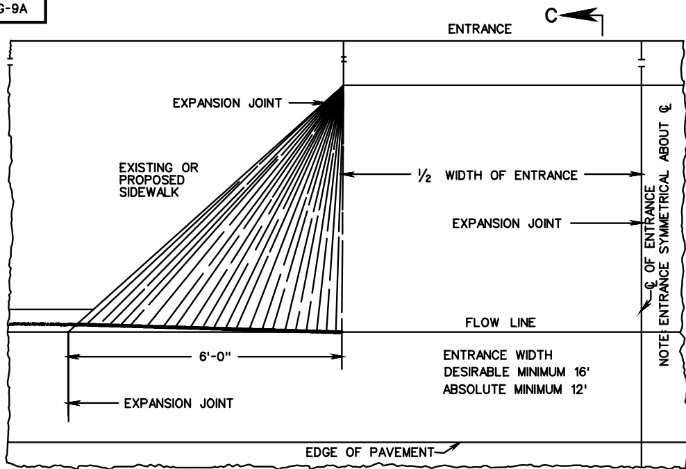
HALF - PLAN
