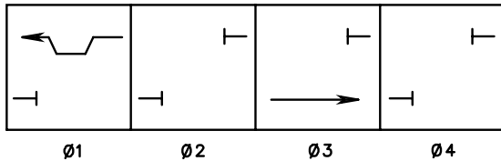
PHASING DIAGRAM
