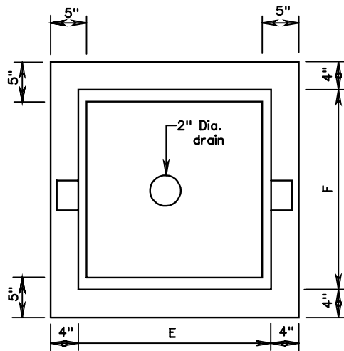
PLAN VIEW (FRAME AND COVER REMOVED)
