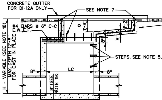
SECTION (CAST IN PLACE)
