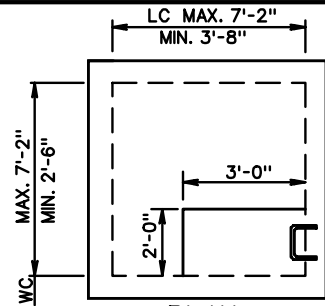
PLAN (SLOT REMOVED)
