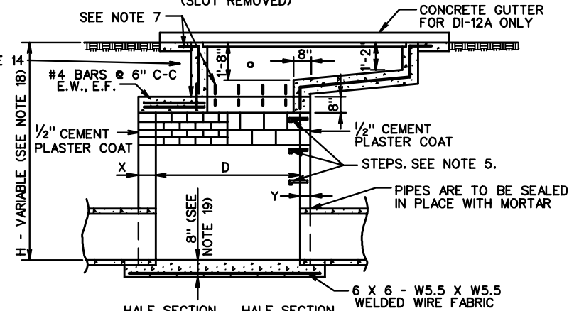
BRICK CONCRETE BLOCK
