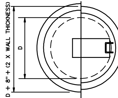
PLAN (SLOT REMOVED)
