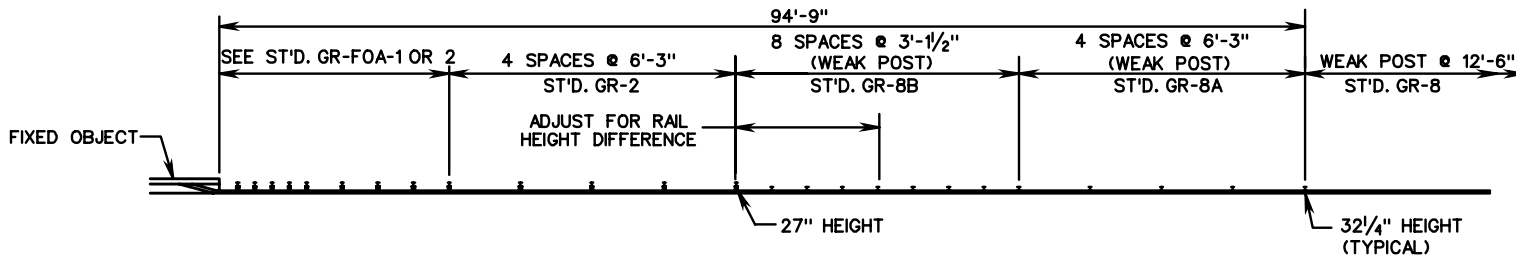
TRANSITION FROM WEAK POST GUARDRAIL TO FIXED OBJECT
