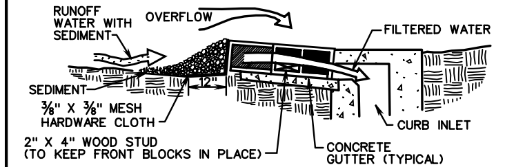
SECTION VIEW
