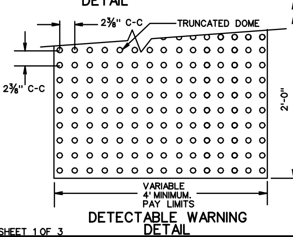
TRUNCATED DOME DETAIL
