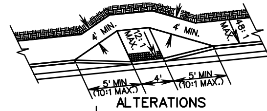
TYPICAL PLACEMENT AT INTERSECTION WITHIN CROSSWALK
