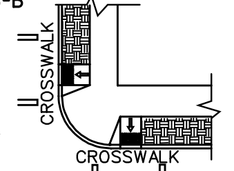
TYPICAL PLACEMENT AT INTERSECTION WITHIN CROSSWALK (WITH BUFFER STRIP)
