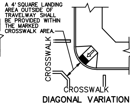
TYPICAL PLACEMENT AT INTERSECTION WITHIN CROSSWALK
