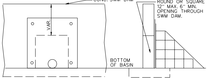
DETAIL FOR METAL PLATE AND WATER QUALITY ORIFICE TYPICAL SWM DAM
