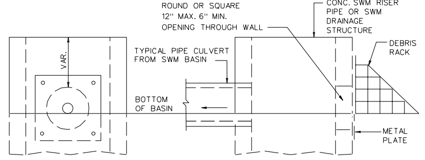
DETAIL FOR METAL PLATE AND WATER QUALITY ORIFICE SIDE VIEW WITH DEBRIS RACK
