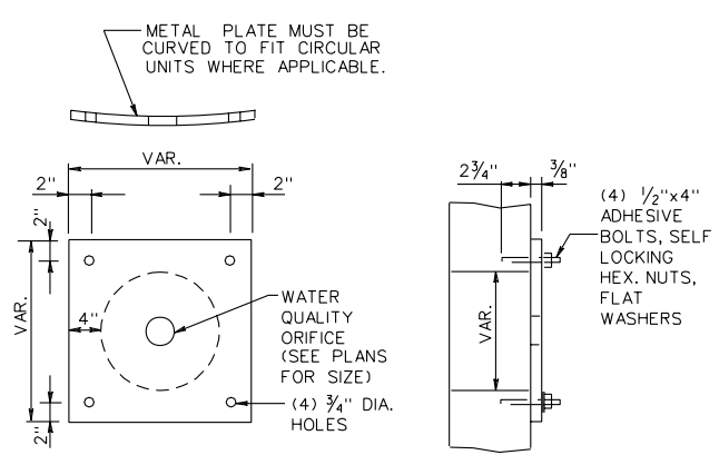
METAL PLATE DETAIL (NOT GALVANIZED)
