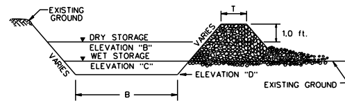
TYPICAL SECTION (AA) THRU TEMPORARY SEDIMENT TRAP
